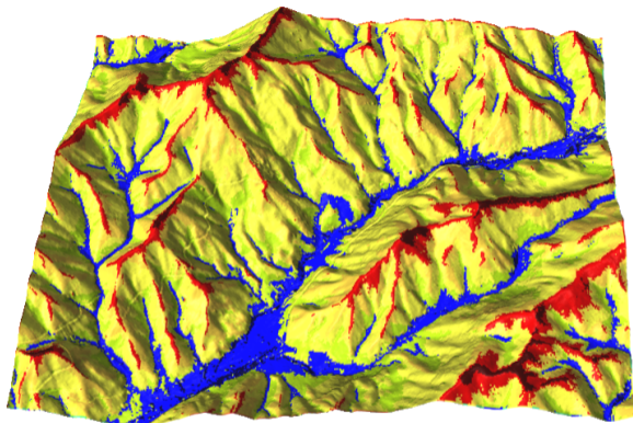
Landforms detected by r.geomorphon
