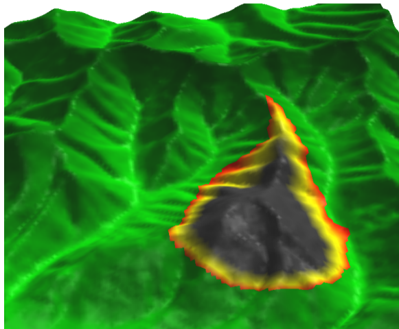
Wildfire spread simulated by r.ros and r.spread
