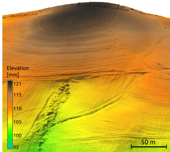
Digital elevation model interpolated by v.surf.rst
