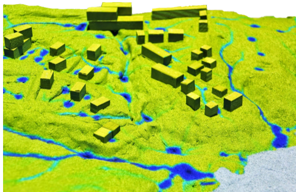
Overland water flow simulated by r.sim.water in Tangible Landscape environment
