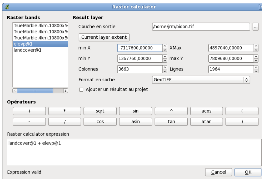
FIGURE 5.2.: Calculatrice raster 🐧
